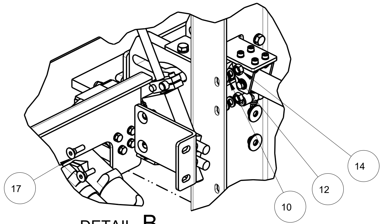
DETAIL B SCALE 5/16
